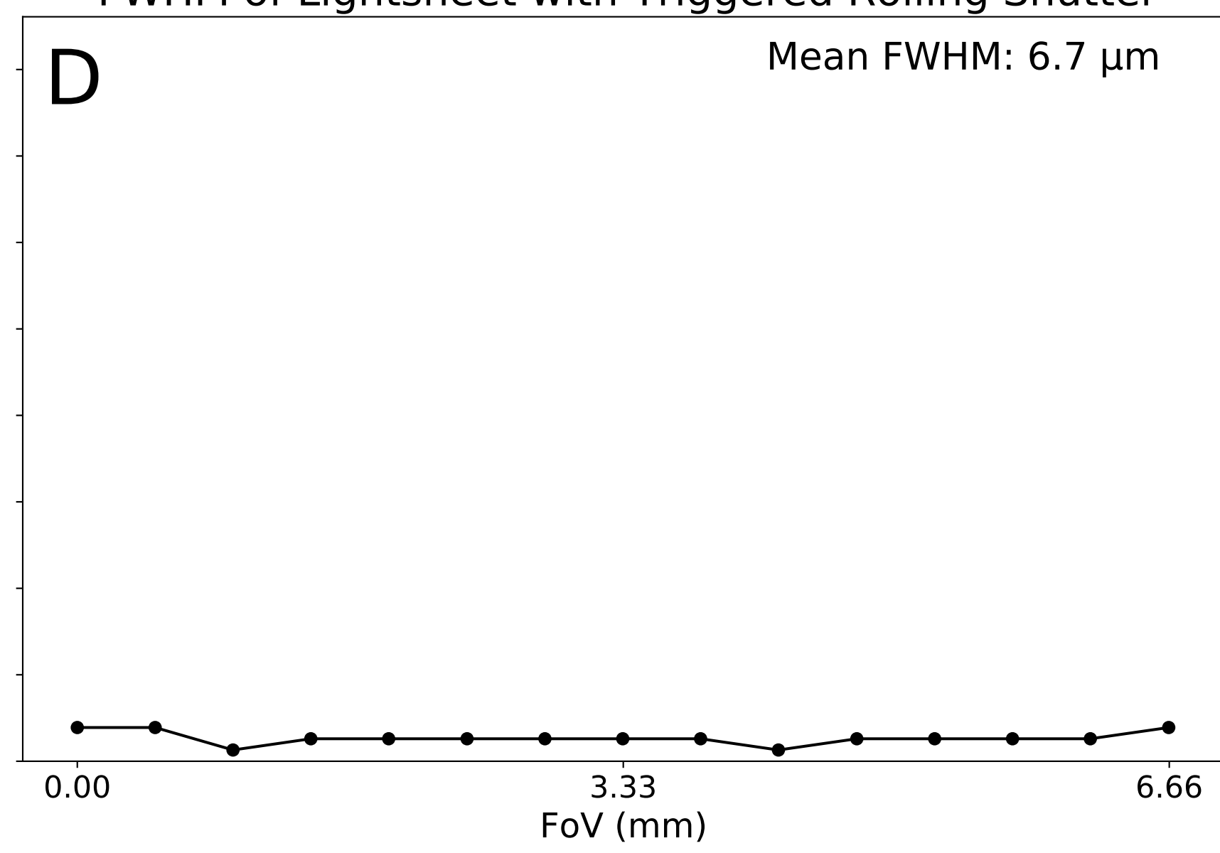
FWHM of Lightsheet with Triggered Rolling Shutter
