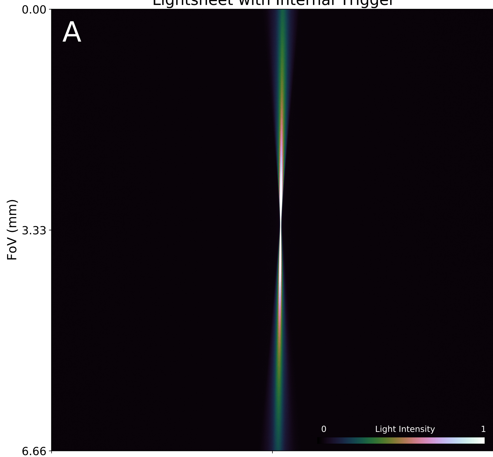
Lightsheet with Internal Trigger
