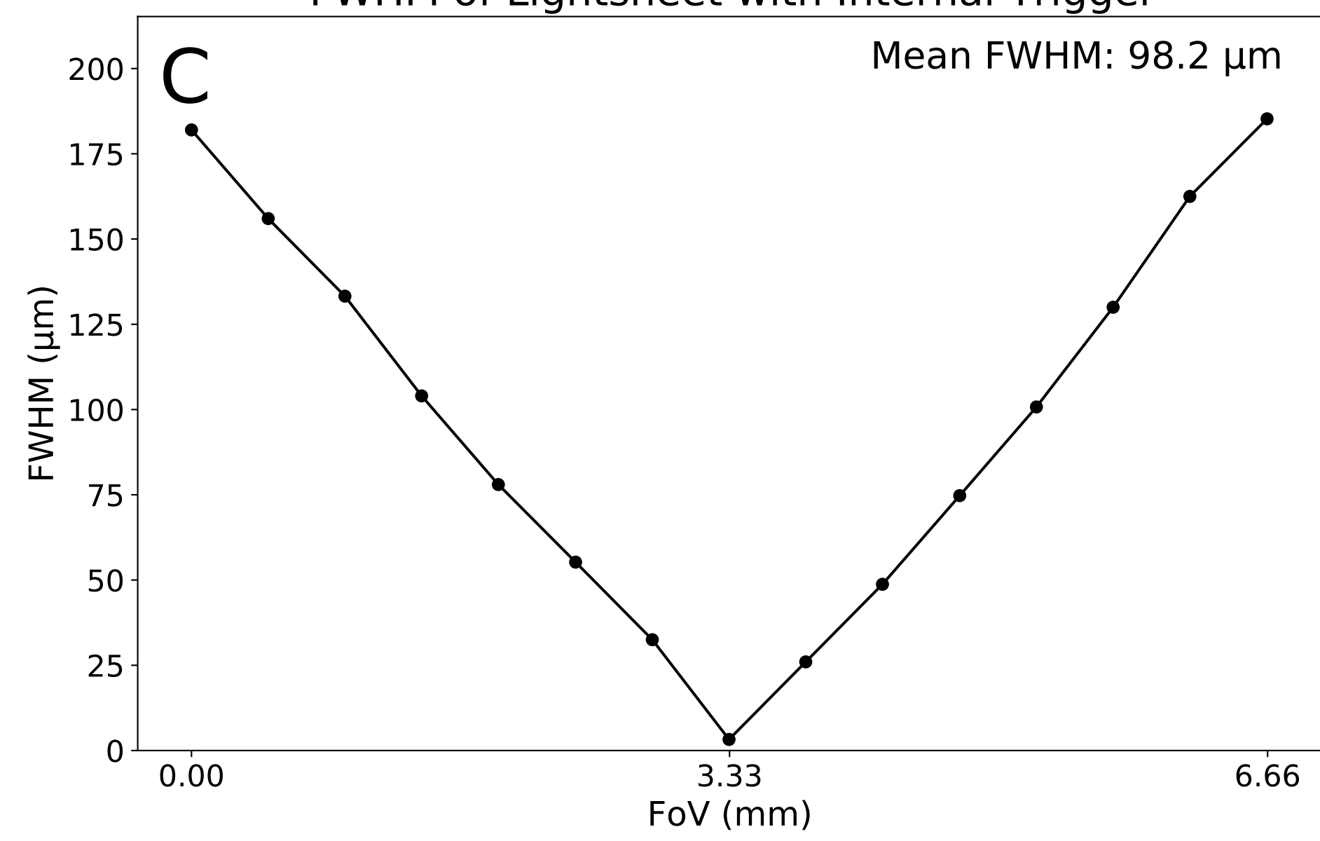
FWHM of Lightsheet with Internal Trigger
