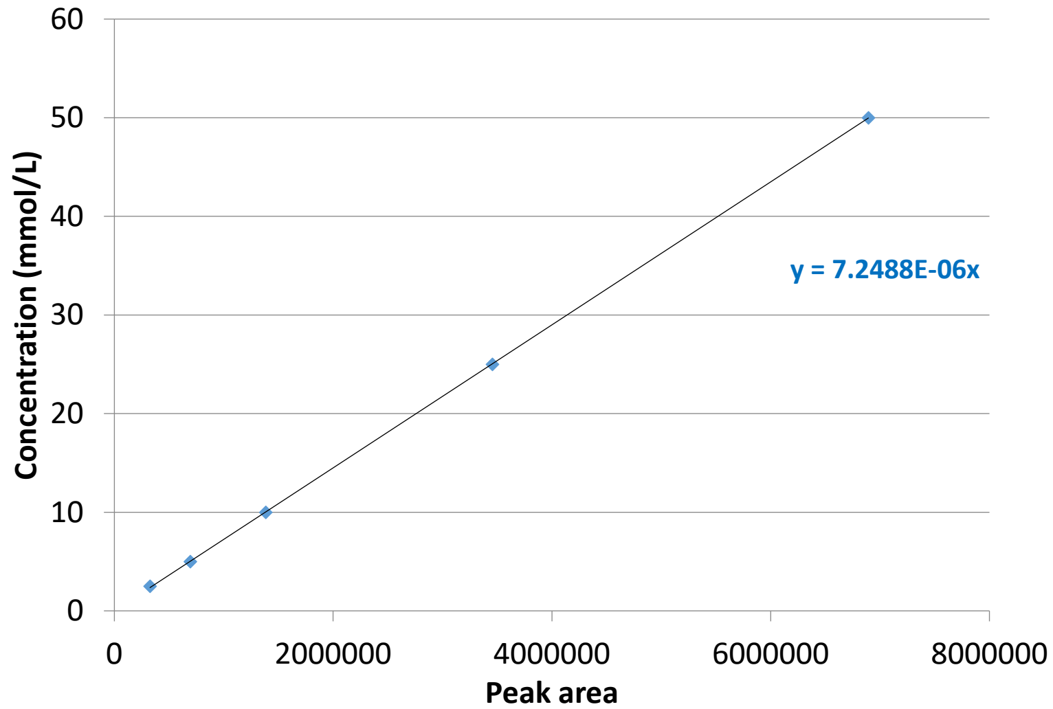
Calibration curve for NB-IPA
