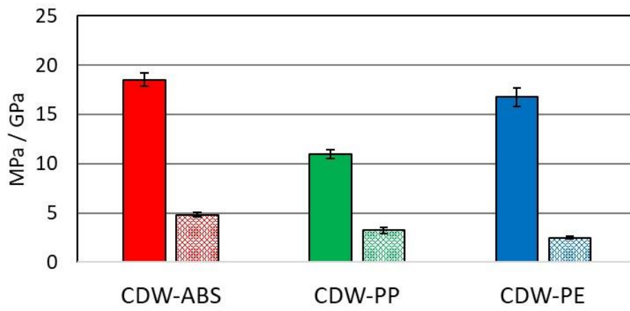
Flexural strength, MPa (solid fill) and flexural modulus, GPa (pattern fill)
