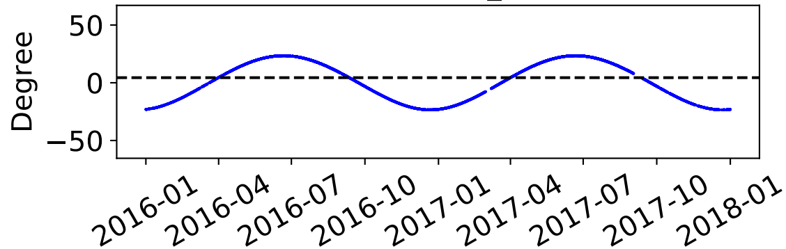
(c) SubStar_Lat
