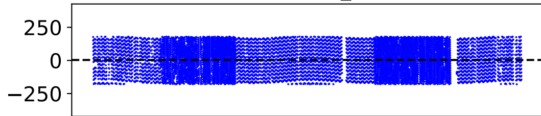
(b) SubObs_Lon
