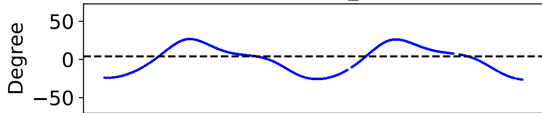
(a) SubObs_Lat
