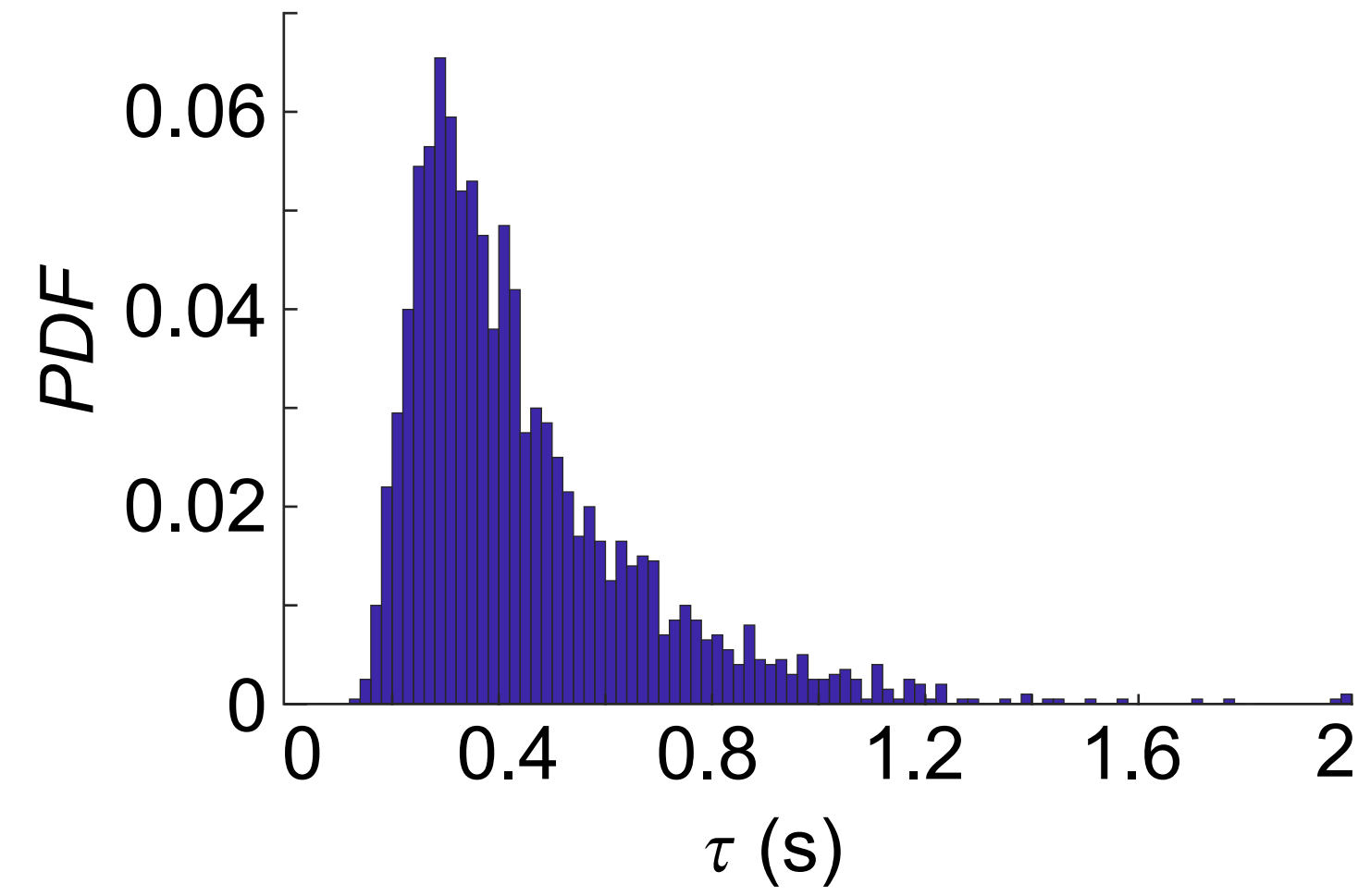
Reorientation time
