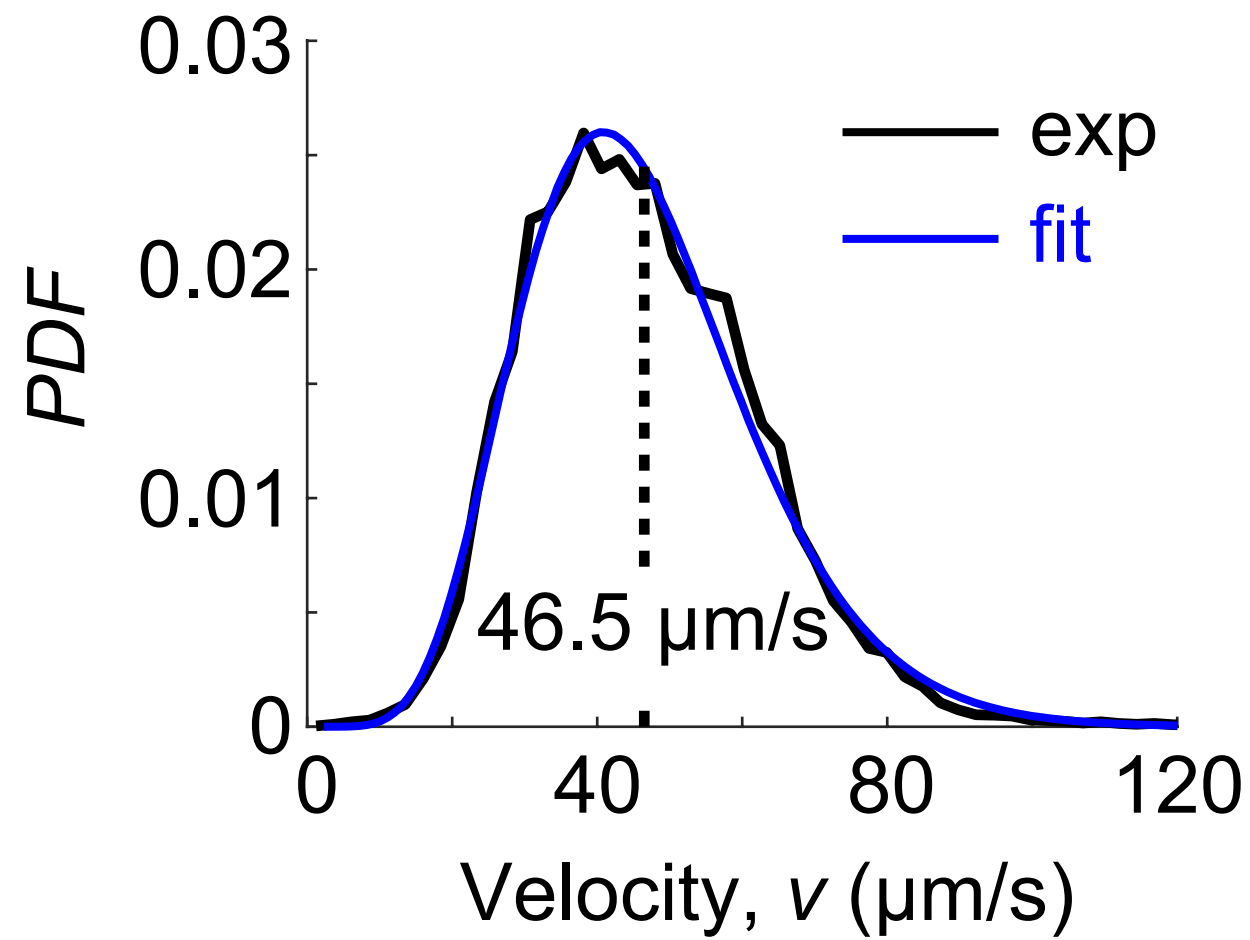
Swimming speed
