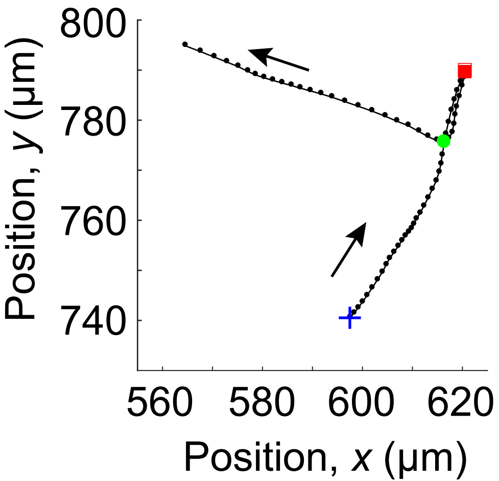
Bacterial tracks
