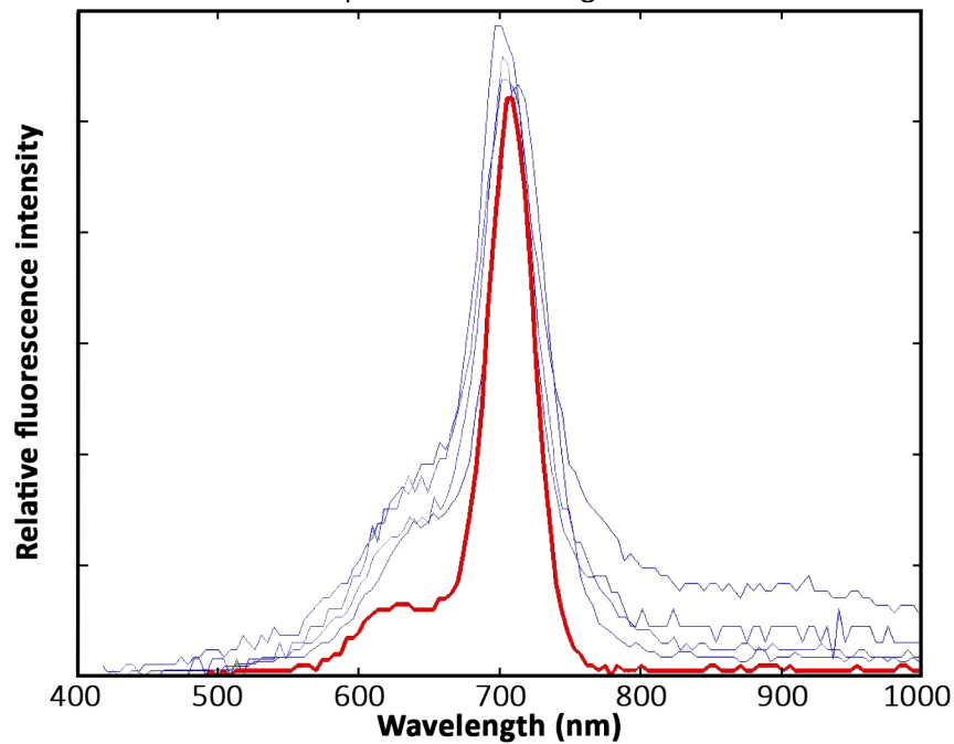
Fluorescence spectrum following 405 nm excitation
