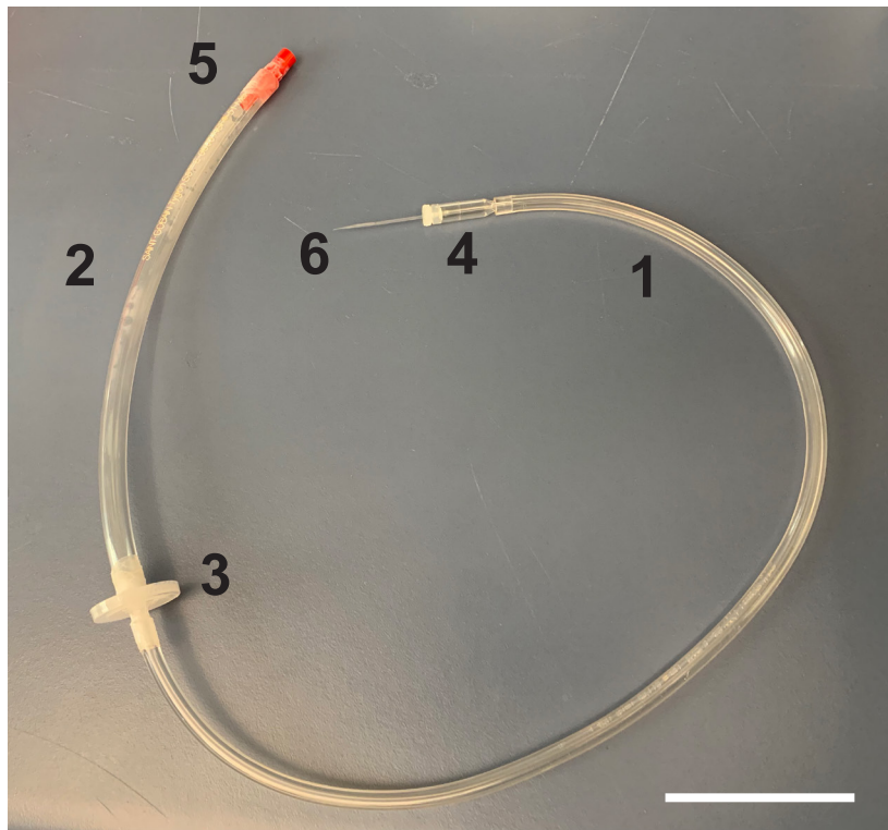
Figure 2. Assembly of mouth pipette
