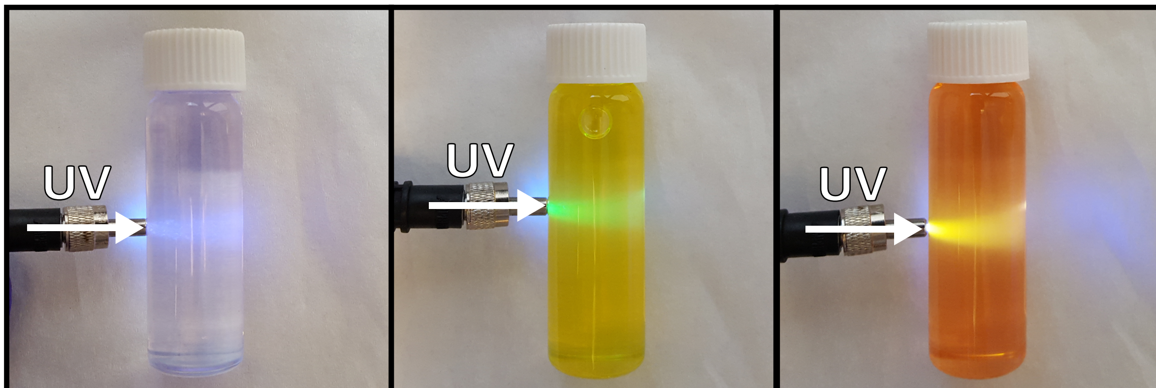
n = 2 MAPbBr
