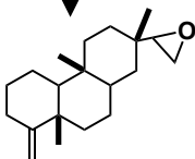
15,16-epoxydolabrene
