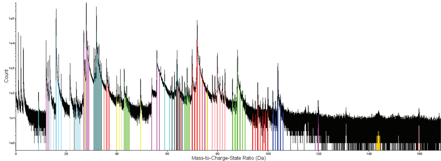
Mass Spectrum
