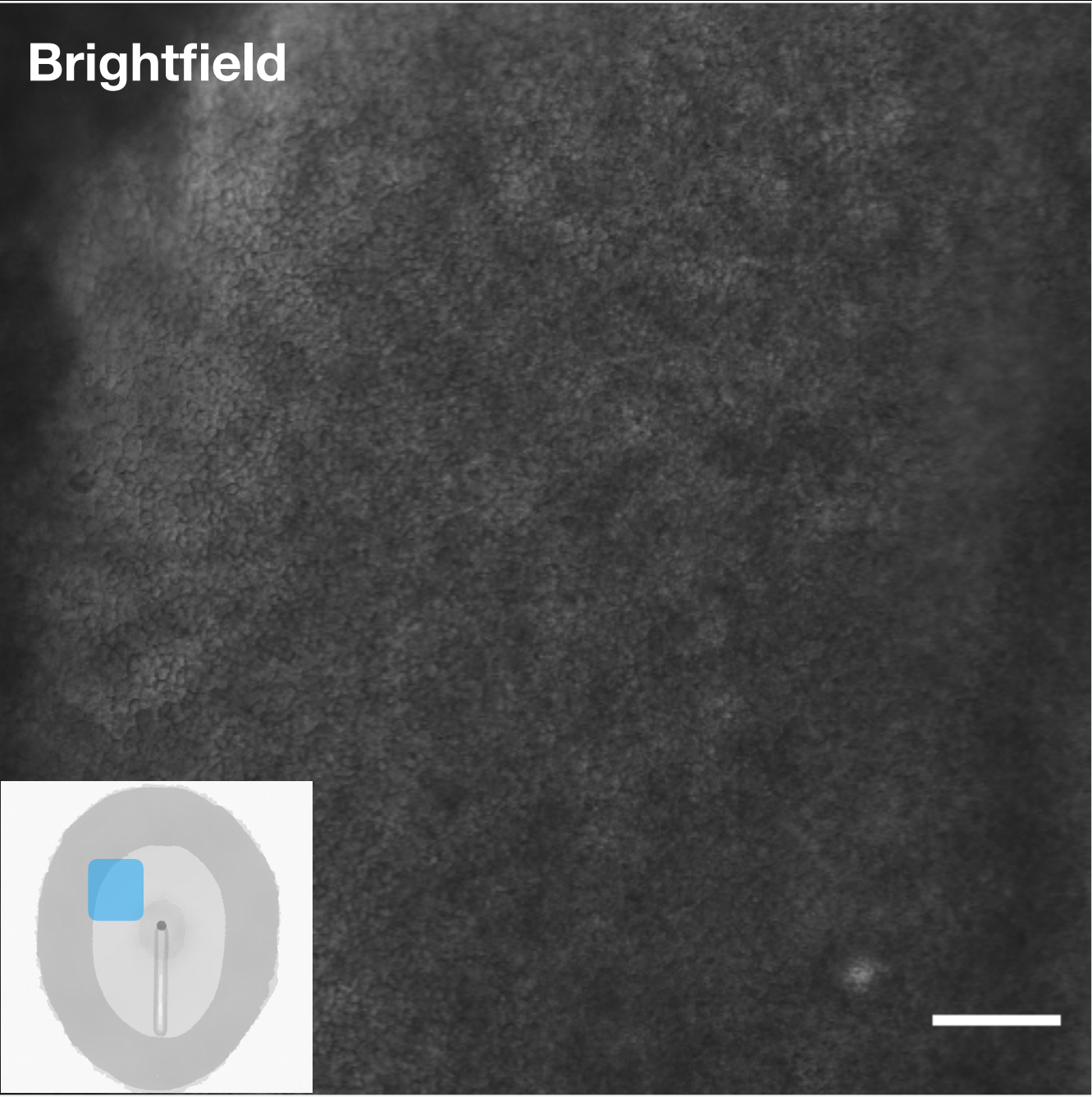
mRNA H2B-Citrine
