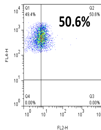
CD19-CAR-T Cells
