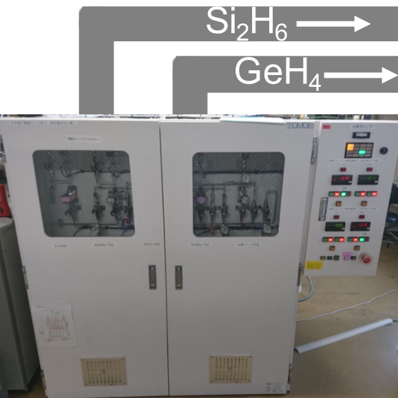
Gas cabinet
