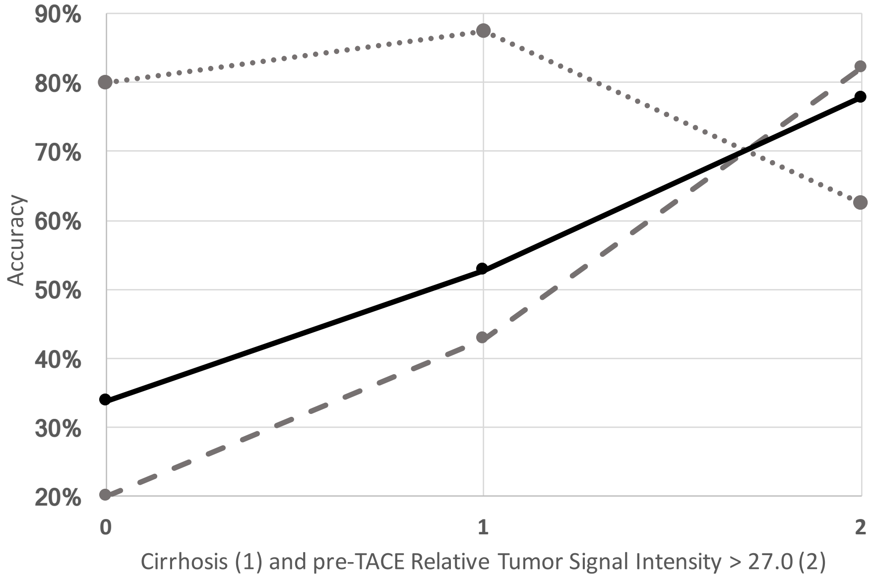
Random Forest Classifier Accuracy vs. Top 2 Features
