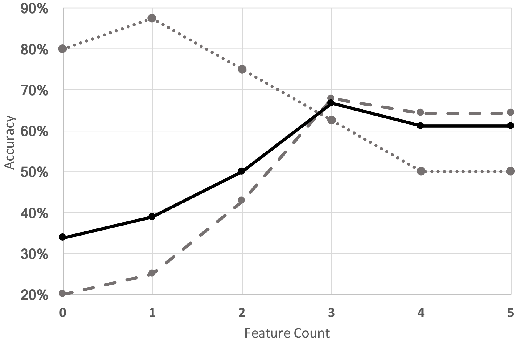
Random Forest Classifier Accuracy vs. Top 5 Features
