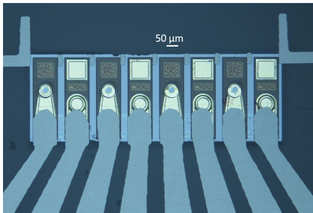
Figure 6: Optical microscope image of a flip-chip bonded VCSEL chip as viewed from the backside of the receiver glass substrate.
