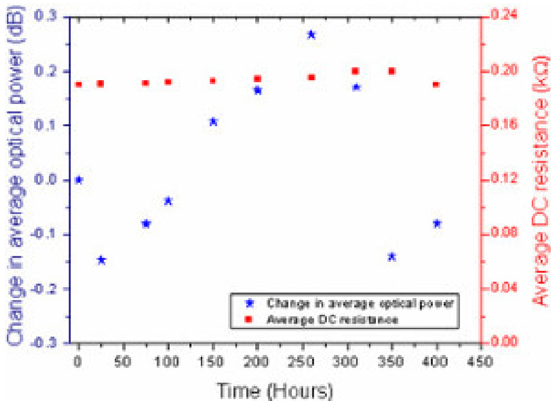
Figure 9: Plot depicting the results of ageing tests performed on the bonded VCSEL chips.
