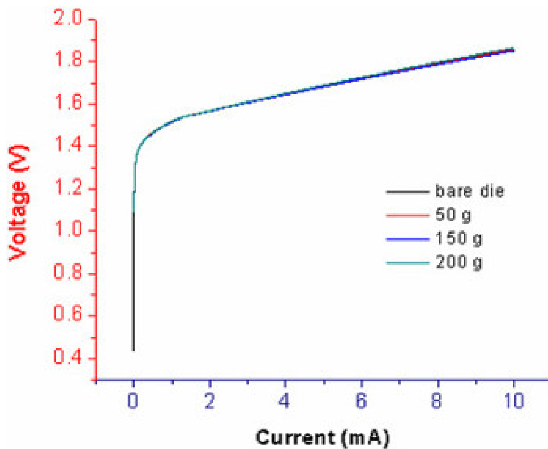
Figure 8: Comparison of I-V curves recorded for flip-chip assemblies bonded using different pressures with those recorded from a bare die. (Modified from 15 )
