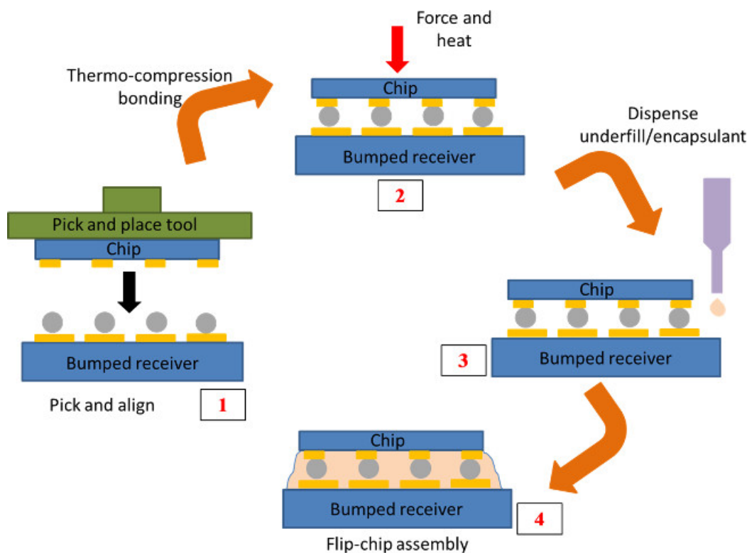
Figure 4: Depicts the various steps involved in the thermo-compression flip-chip bonding of OE components.
