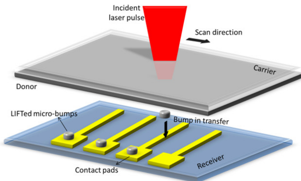
Figure 1: Schematic illustrating the principle of the LIFT technique.
