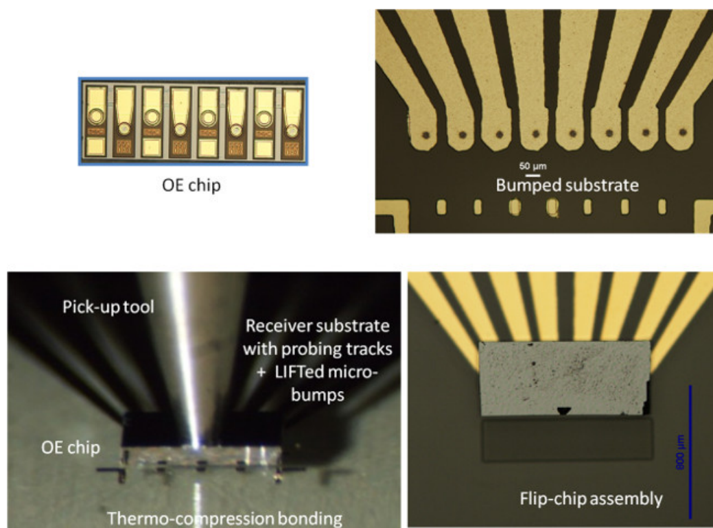
Figure 5: Optical micrographs taken at various processing steps.
