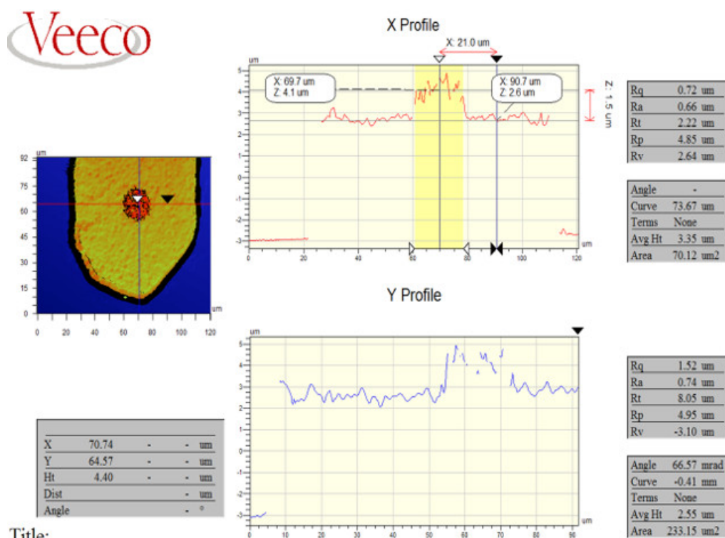
Figure 3: Typical optical profilometer measurements of the LIFTed micro-bumps.
