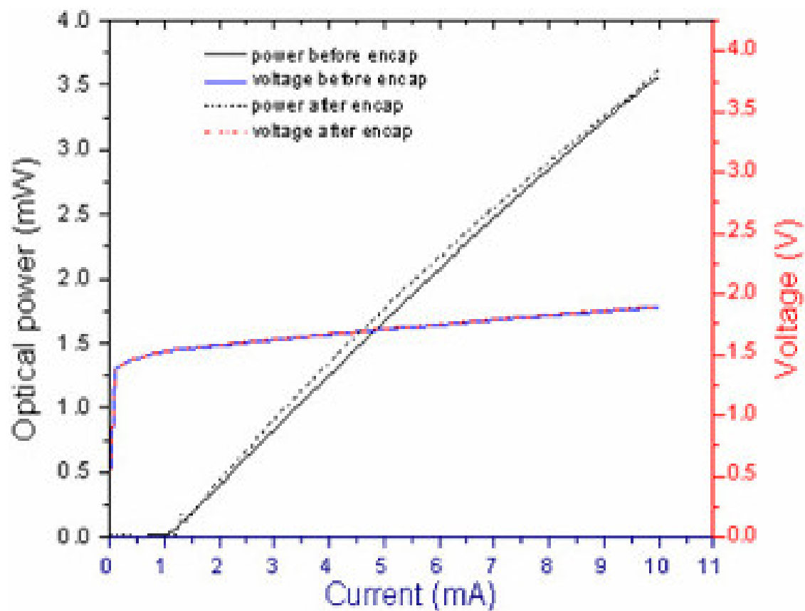
Figure 7: Typical LIV curves recorded for a flip-chip VCSEL assembly prior and post encapsulation. (Modified from 15 )
