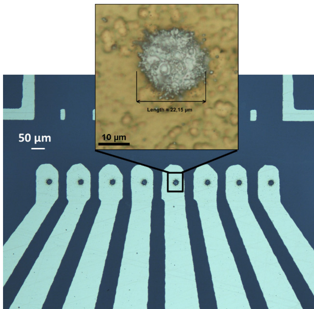
Figure 2: Optical micrograph of a LIFT-assisted bumped receiver substrate. The inset shows a magnified image of a printed indium micro-bump.
