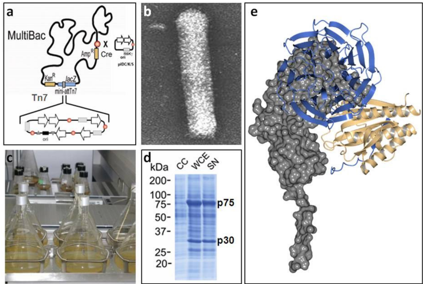
Figure 1: MultiBac platform technology for multiprotein complex production.
